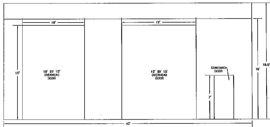
FRONT VIEW
