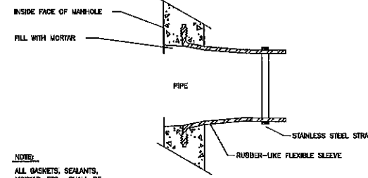
DETAIL "A" - PIPE TO MANHOLE JOINTS
