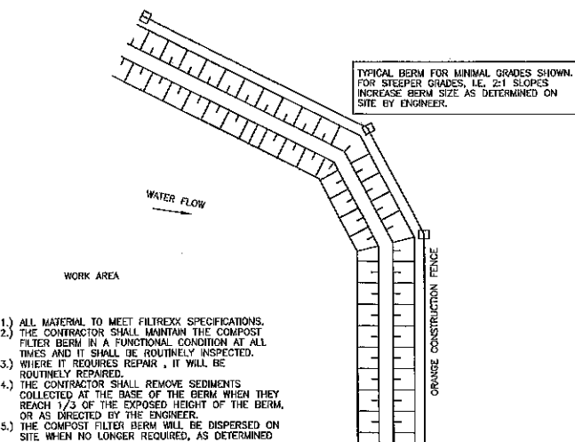
7 FILTERREXX SOCK - SILT FENCE NOT TO SCALE
