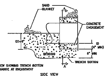
SECTION A-A (SEE NOTE 10)
