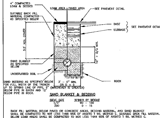
⑥ WATER LINE TRENCH NOT TO SCALE
