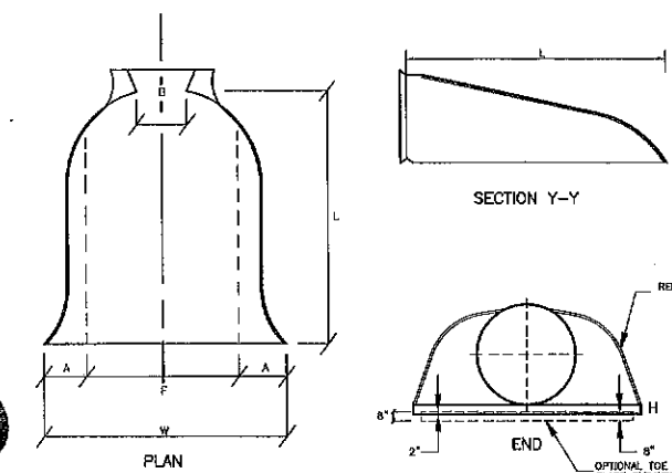
⑧ RIPRAP DETAIL NOT TO SCALE
