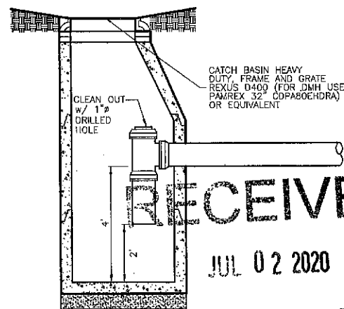
6 DEEP SUMP HOODED CATCH BASIN NOT TO SCALE
