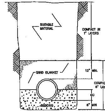
TRENCH CROSS-SECTION NOT TO SCALE
