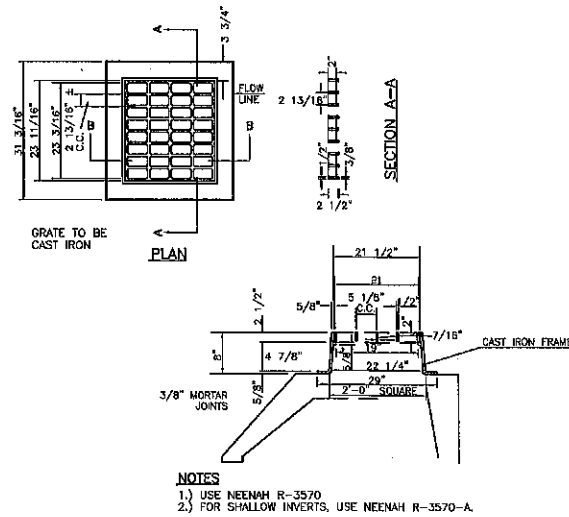
① CATCH BASIN FRAME & GRATE NOT TO SCALE
