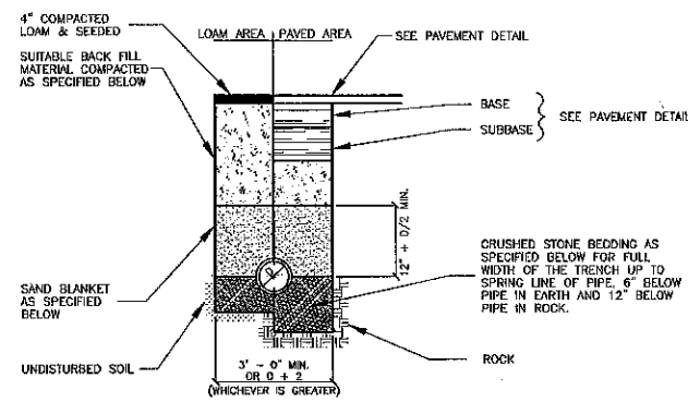
⑥ WATER LINE TRENCH NOT TO SCALE
