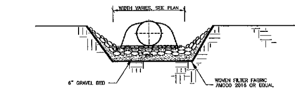
⑧ RIPRAP DETAIL NOT TO SCALE
