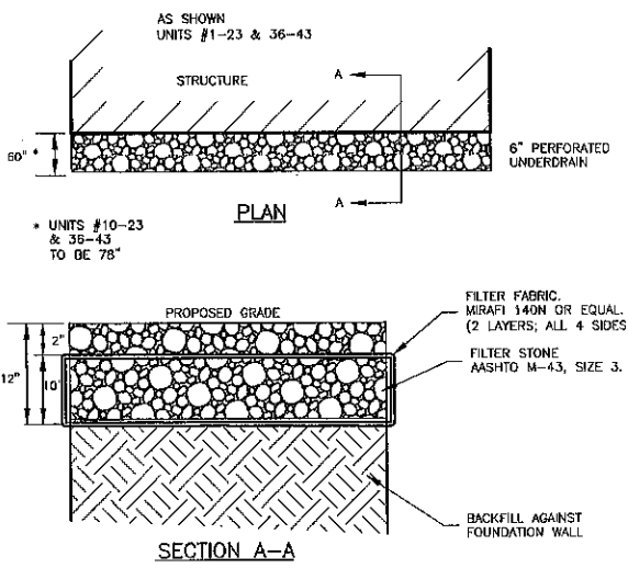
10 BUILDING DRIP EDGE NOT TO SCALE
