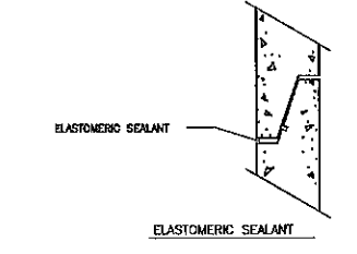
DETAIL "B" - HORIZONTAL JOINTS
